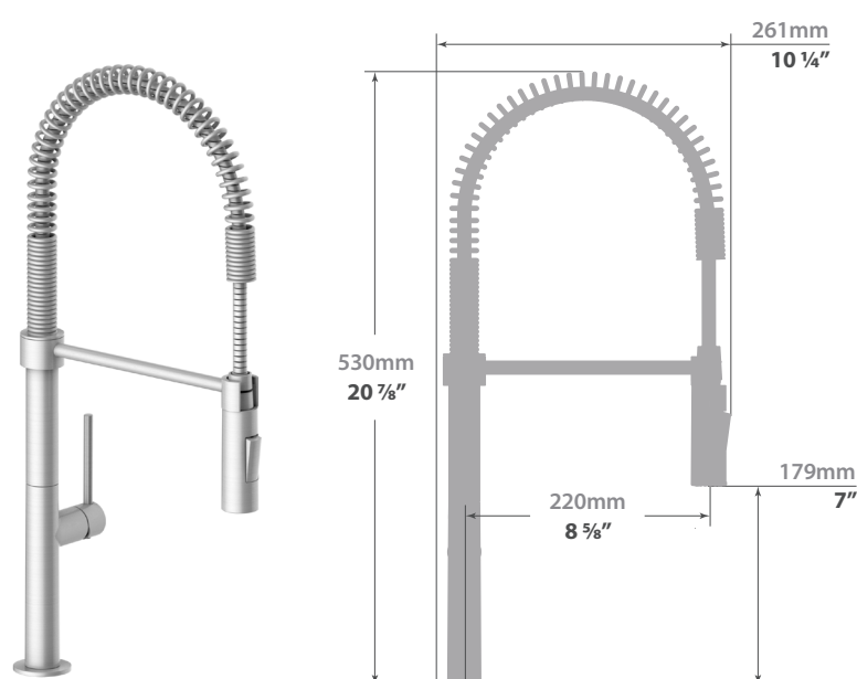
360° Swivel Spout
